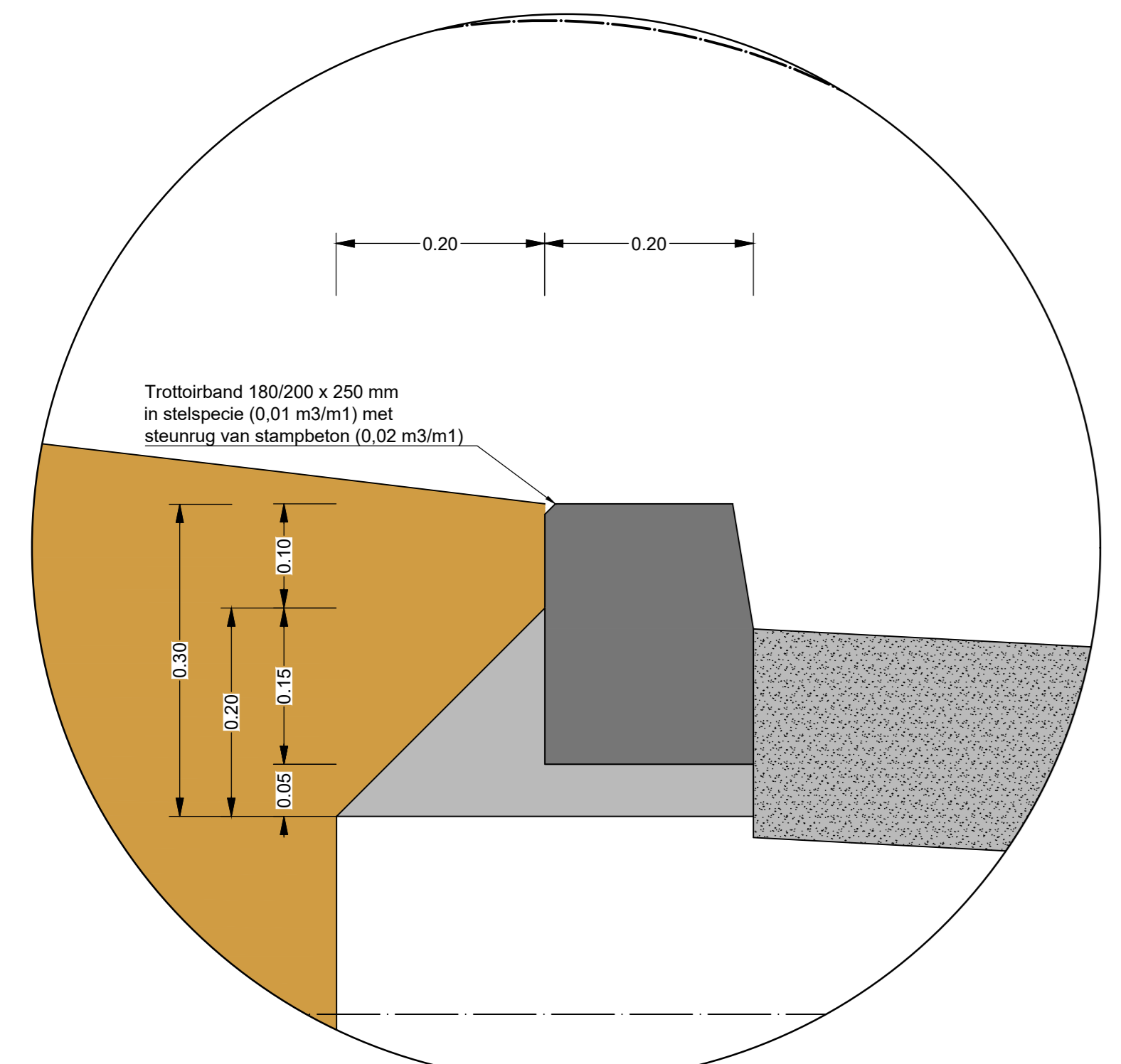
Detail 1, principe detail Schaal 1:5
