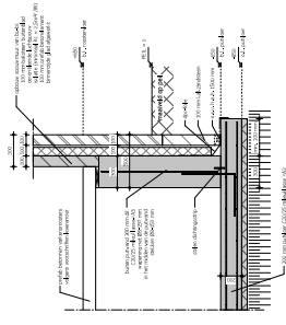
DETAIL H
