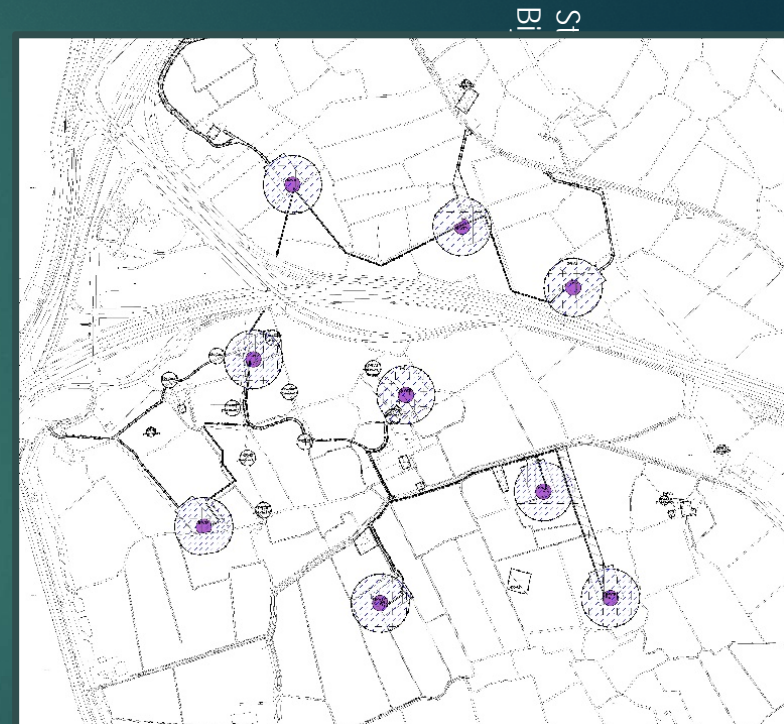
Palenplan windpark NHH
