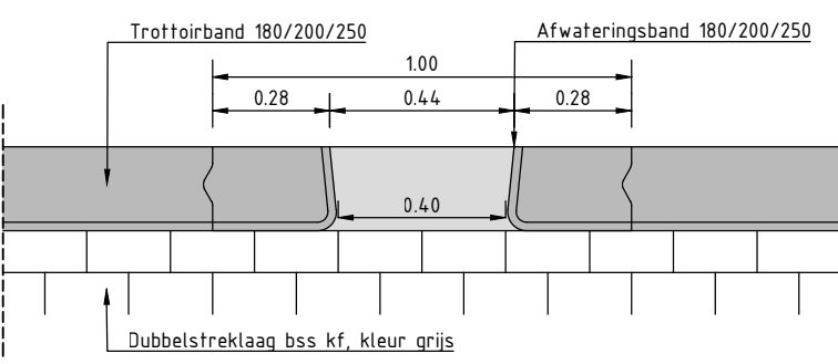
Principe detail 01: afwateringsopeningen h.o.h. 3m Schaal 120
