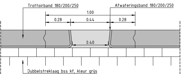
Principe detail 01: afwateringsopeningen h.o.h. 3m Schaal 120
