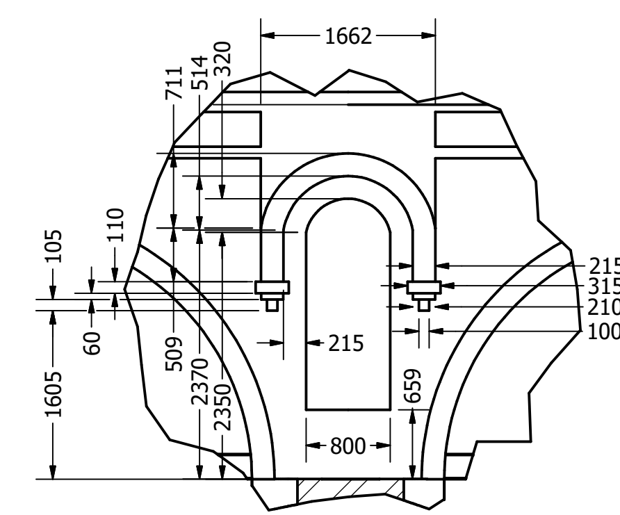
DETAIL G SCALE 1 / 50 Middennis
