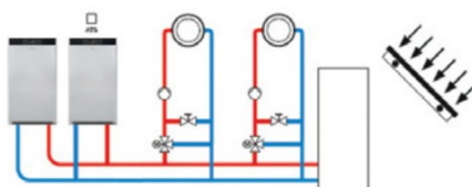
Vitotronic 300-K (multi boiler) Weather compensation cascade control allowing the control of 4 boilers equipped with Vitotronic 100.
