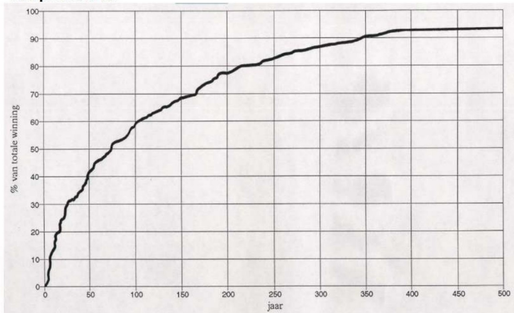
Figuur 4-3 Responsecurve van de winning Garyp (Vitens, 2010)
