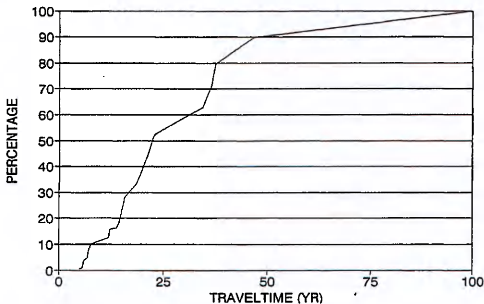
Figuur 4-3 Responsecurve van de winning Ameland Hollum (Vitens, 2010)
