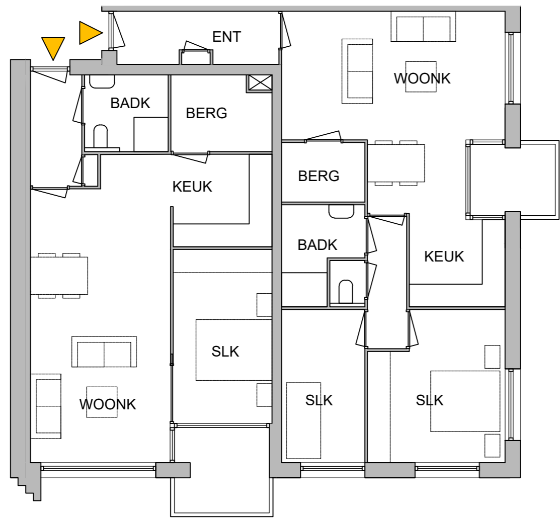
1-G BASIS TWEEKAMER WONING
