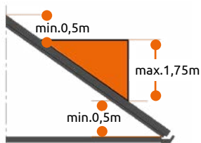
Normale dakkapel
