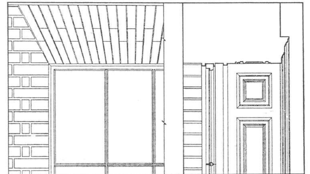
55 Already recessed four inches under the Act of 1709, window frames were now, under the Building Act of 1774, further concealed behind brick reveals, leaving only a tiny margin of woodwork to catch fire and spread conflagration in the street.
