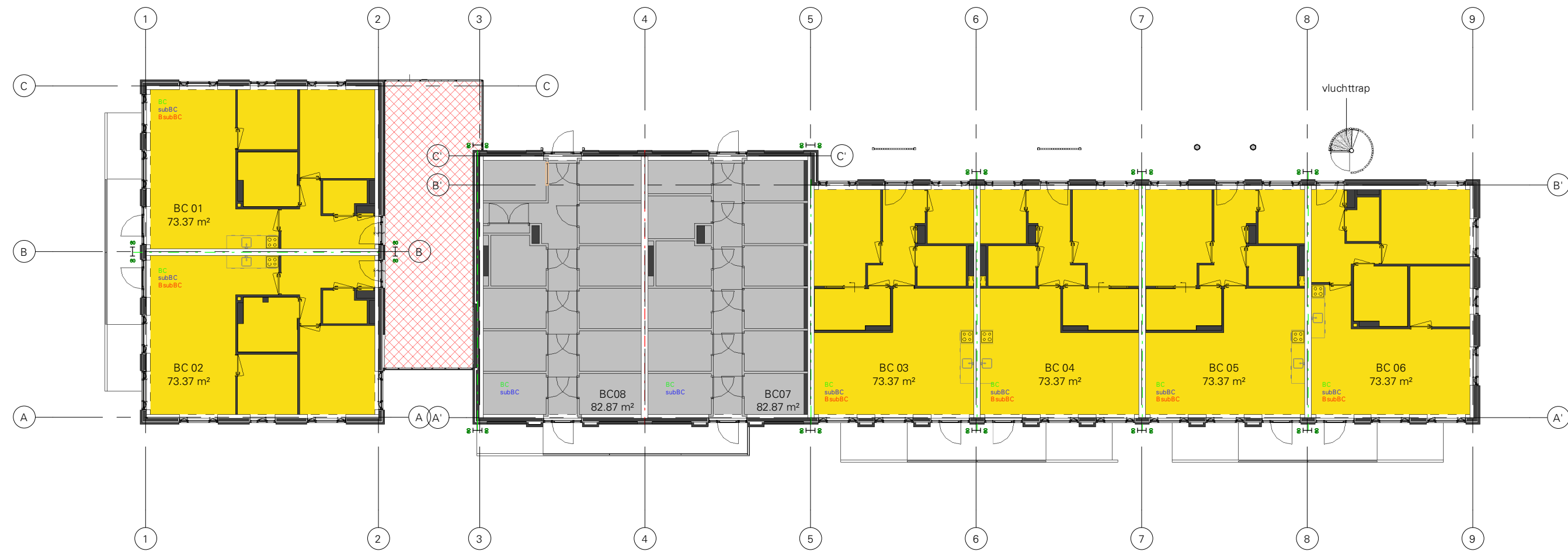
00 begane grond
